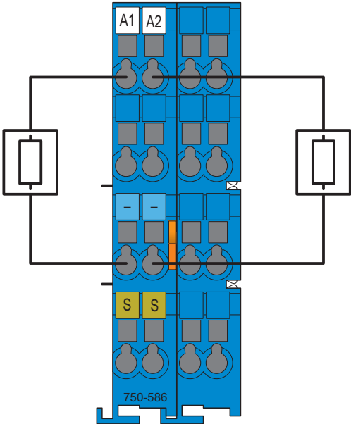
Figure 12: Connecting diagram
