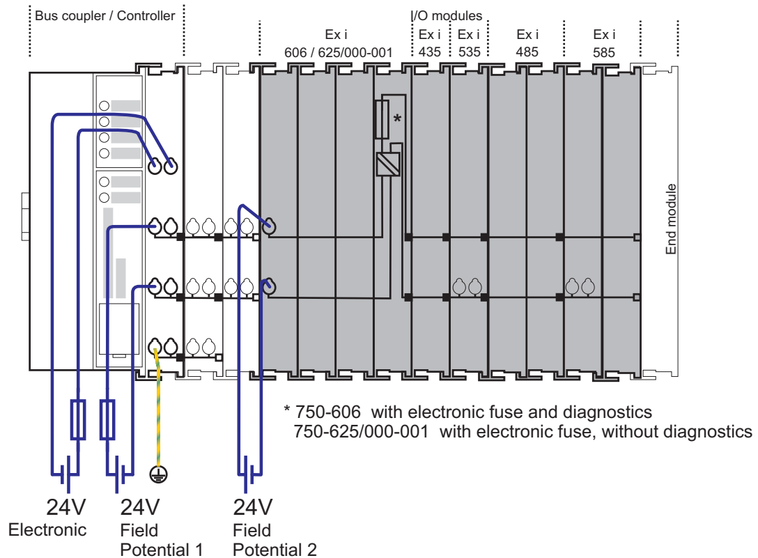
Figure 1: Supply Principle Ex i
