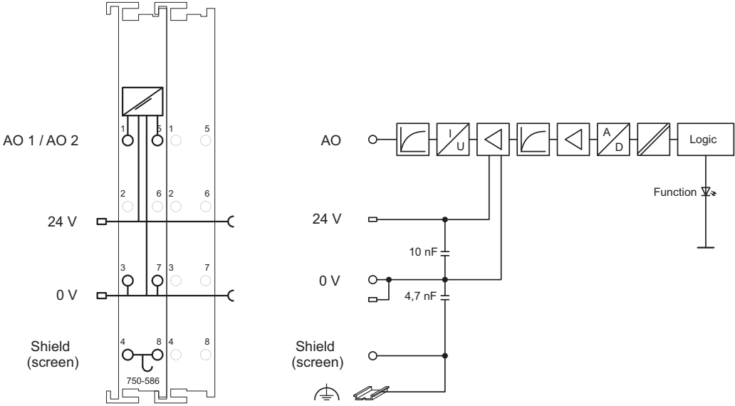
Figure 7: Schematic diagram
