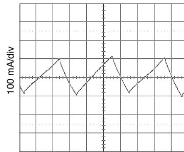
1 \mu s/div 5 V_{IN} , 3.3 V_{OUT} , 5 A load MFP0507S Input Ripple ( I_{IN} ) FIGURE 14
