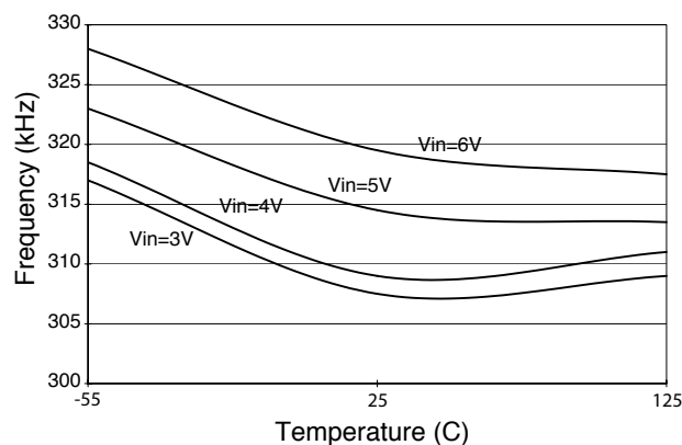
FIGURE 20 TYPICAL OPERATING FREQUENCY VS TEMPERATURE AND V_{IN}
