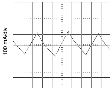
1 \mu s/div 3.3 V_{IN} , 1.2 V_{OUT} , 5 A load MFP0507S Input Ripple ( I_{IN} ) FIGURE 13
