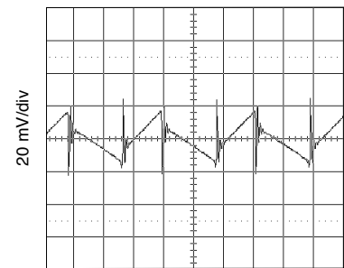
1 \mu s/div 3.3 V_{IN} , 1.2 V_{OUT} , 5 A load MFP0507S Output Ripple FIGURE 15
