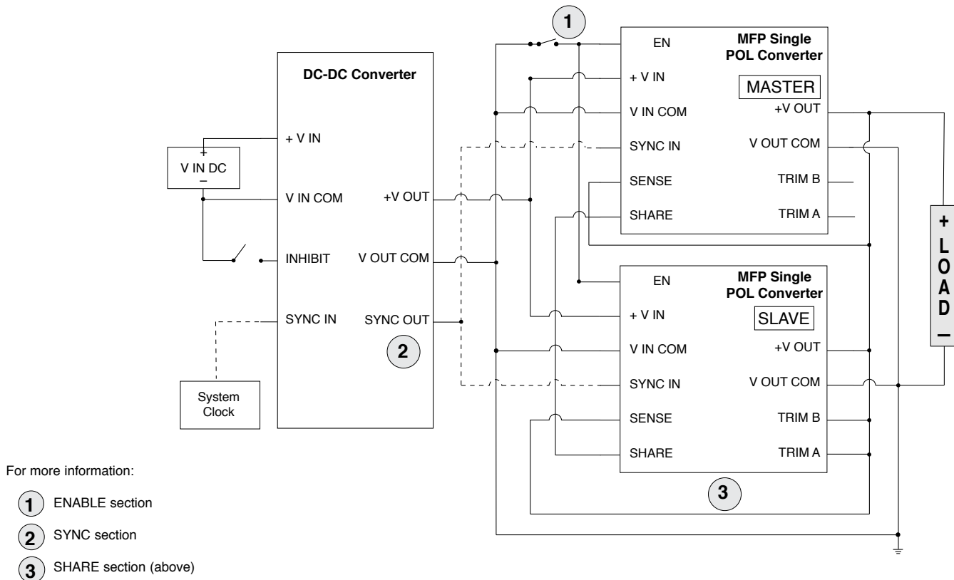
FIGURE 10: TYPICAL SHARE CONNECTION WITH OPTIONAL SYNC
