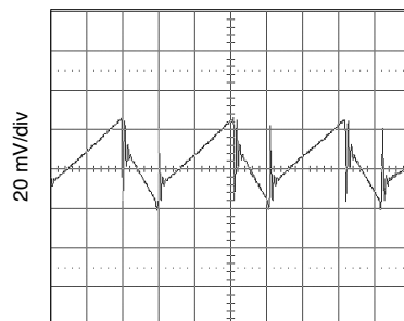
1 \mu s/div 5 V_{IN} , 3.3 V_{OUT} , 5 A load MFP0507S Output Ripple FIGURE 16
