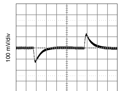
200 \mu s/div 5 V_{IN} , 3.3 V_{OUT} , 5 A load MFP0507S Load Transient FIGURE 18
