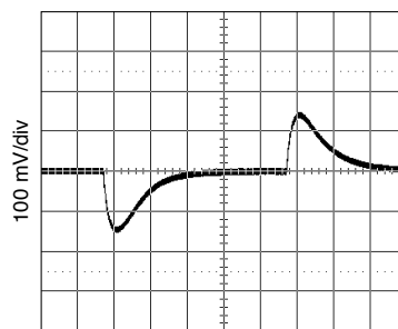
200 \mu s/div 3.3 V_{IN} , 1.2 V_{OUT} , 5 A load MFP0507S Load Transient FIGURE 17
