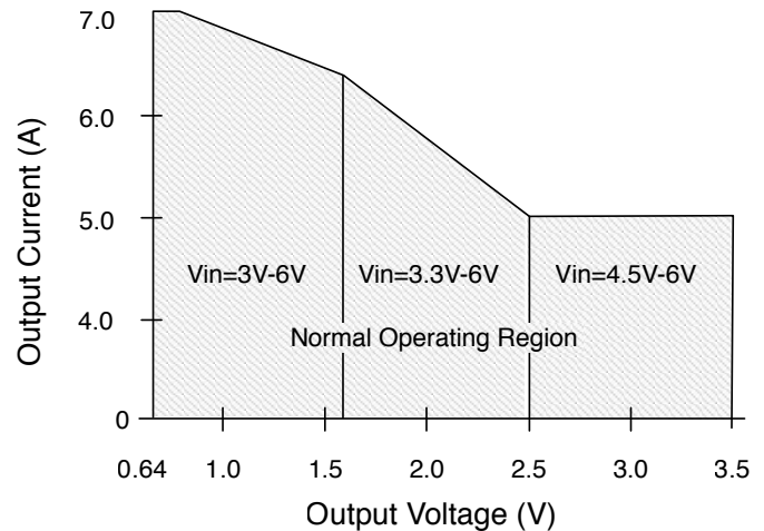
FIGURE 11: MAXIMUM RATED OUTPUT CURRENT
