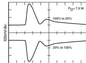
SMHF2815D VOUT STEP LOAD RESPONSE
