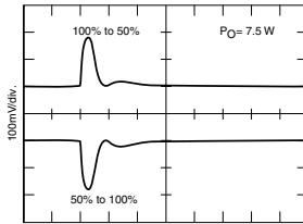
SMHF2805S STEP LOAD RESPONSE
