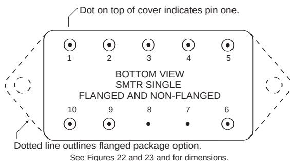
FIGURE 3: PIN OUT SINGLE OUTPUT MODELS
