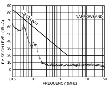
Three paralleled and synchronized MFL2815D converters with an FME28-461. FIGURE 9
