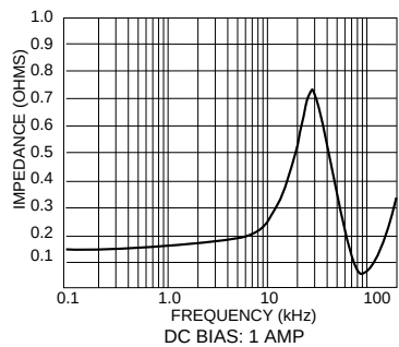
FME28-461 OUTPUT IMPEDANCE FIGURE 10
