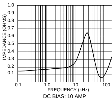
FME28-461 OUTPUT IMPEDANCE FIGURE 11
