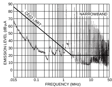
Three paralleled and synchronized MFL2815D converters without filtering. FIGURE 8
