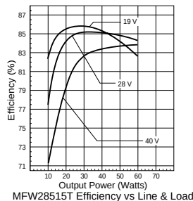
MFW28515T Efficiency vs Line & Load
